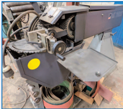
FEIN GX 752H STATIONARY BELT GRINDER
