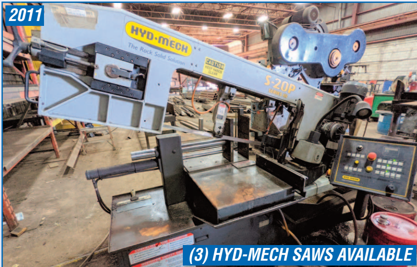
HYD-MECH S-20P SERIES III SEMI-AUTO HORIZONTAL PIVOT BANDSAW
